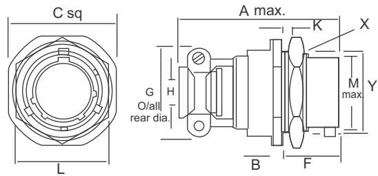
62 IN - 14F Single hole mounting with grommet and grommet nut with integral strain relief clamp has panel 'O' ring seal
