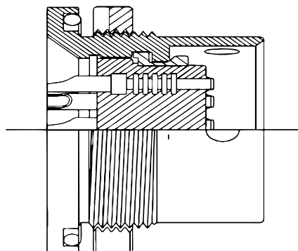
164-127/U Plug With Rigid Contacts, Solder Pocket Terminal, Right Angled Rear Shell
