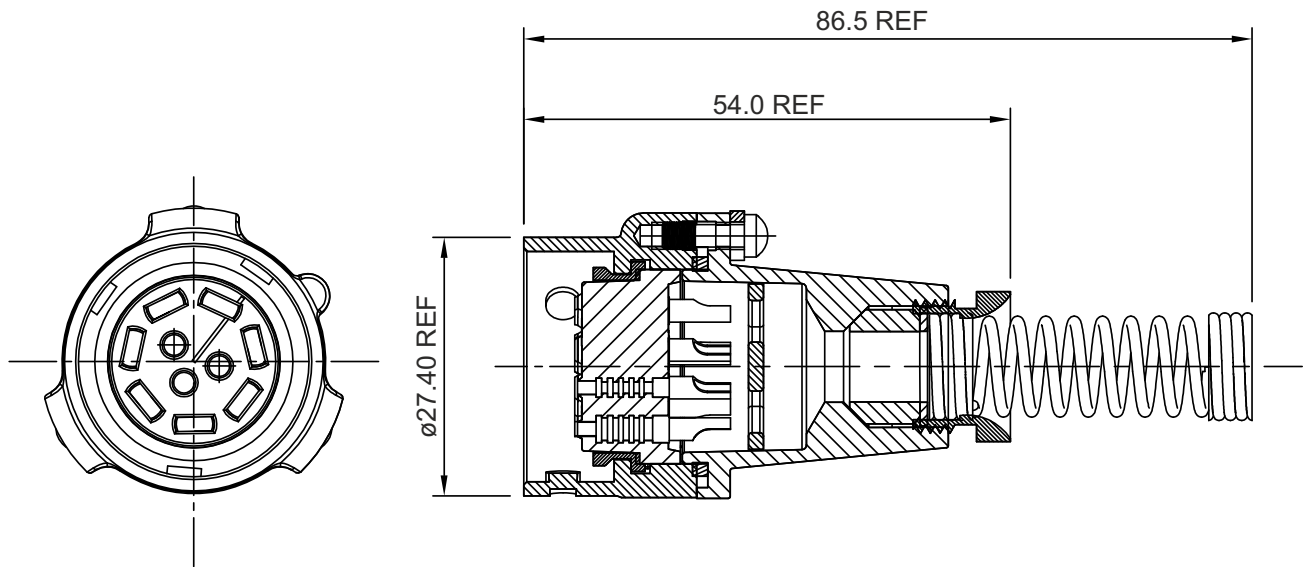
164-78/U Receptacle With Non Rigid Contacts, Solder Pocket Terminal, Straight Rear Shell
