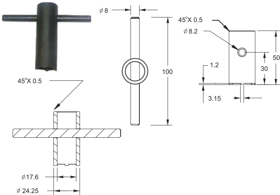
Tightening Spanner (164-T002) (Panel Nut Tightening For 164-183 Connector - Torque Wrench Provision)
