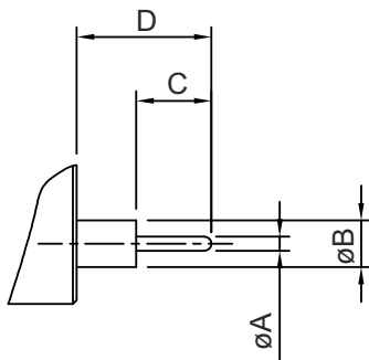
164-79/U—PL—XX STEPPED PIN DESIGN
