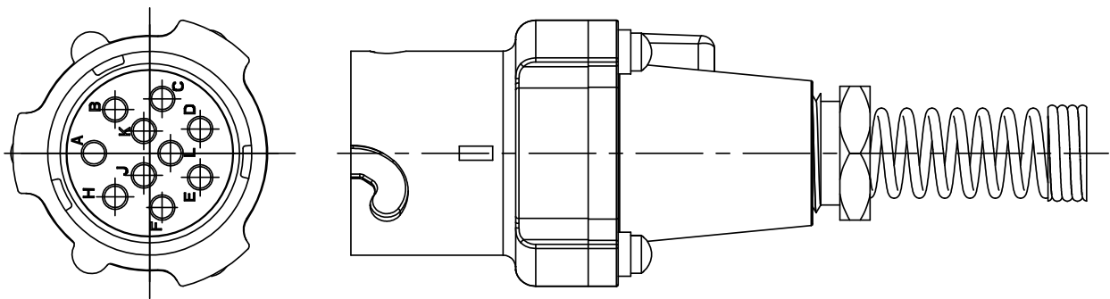
164-79/U Panel Mount Receptacle With Non Rigid Contacts, Solder Pocket Terminal
