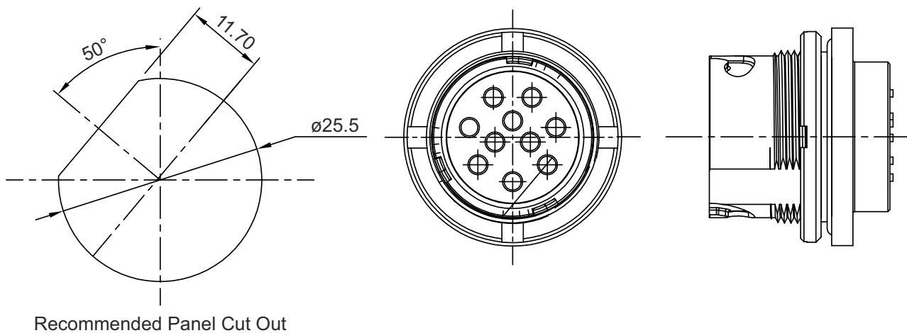
164-79/U Panel Mount Receptacle With Non Rigid Contacts, Solder Pocket Terminal
